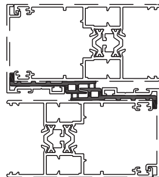
RTC-106P Perfil Engate PVC - RTC-46
