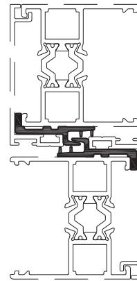
RTC-105P Perfil Engate PVC - RTC-38
